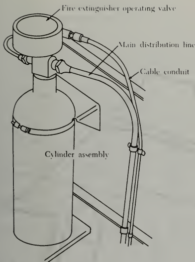
FIGURE 9-8. CO 2 cylinder installation.
